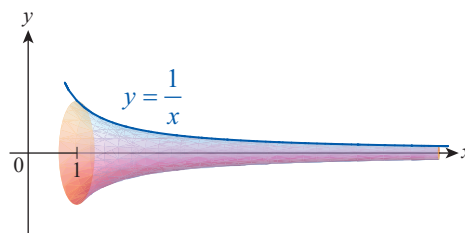
Gabriel's Horn
