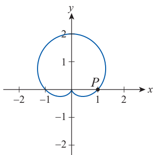
Cardioid
