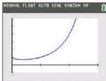
Figure 3 y = x^x on [0, 3] by [-1, 6]
